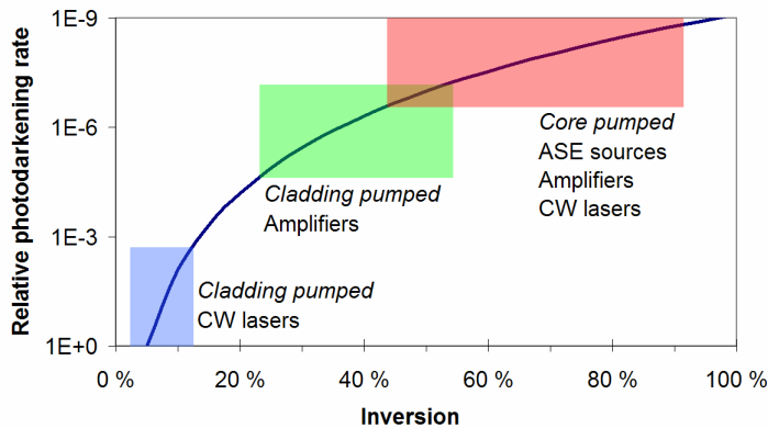
Figure 2. Normalized photodarkening rate as a function of inversion, assuming a 7 th -order power law. Device application regions with different inversion levels are highlighted.
