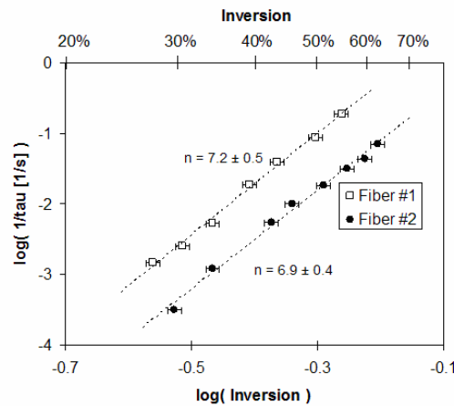
Figure 1. Measured photodarkening rate constant as a function of inversion. The slope of the log-log plot indicates a 7 th order power dependence.
