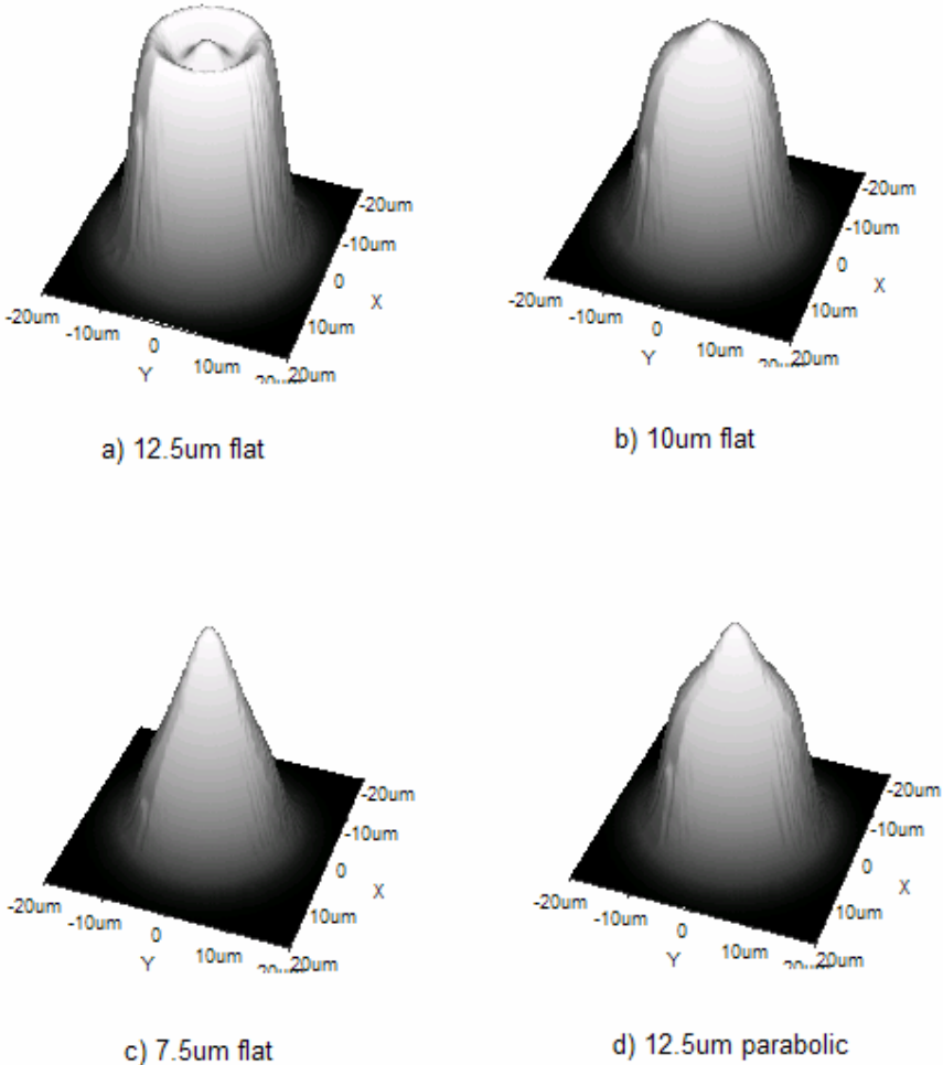
Figure 4: Profiles of the output beams for the ytterbium doped fiber
