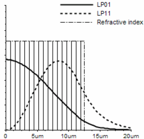
Figure 5: The normalized intensity modal distribution at 1550 nm for 12.5 \mu\text{m} core radius with \text{NA}=0.06
