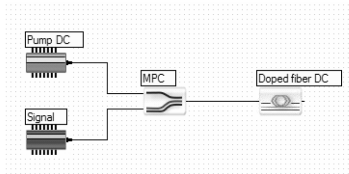
Figure 1: The setup used in simulations
