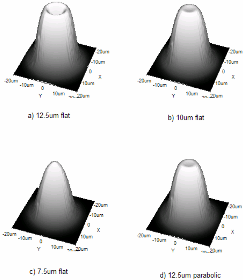
Figure 7: Profiles of the output beams for the erbium doped fiber
