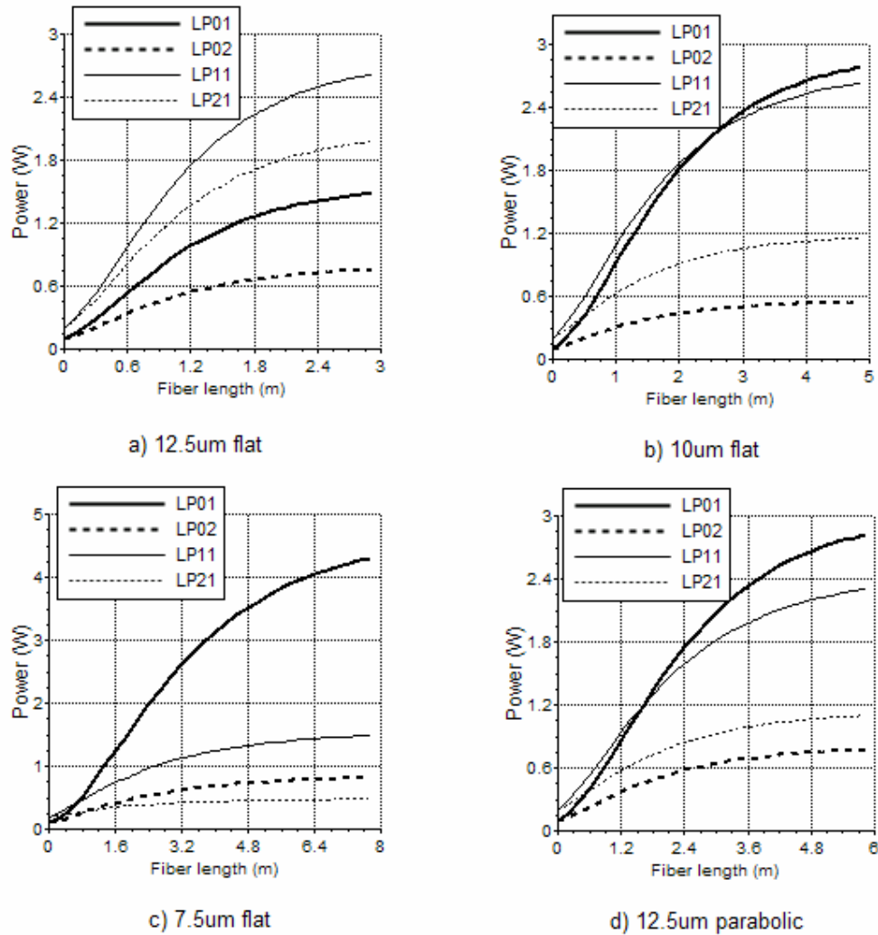
Figure 3: Propagation of individual modes in the ytterbium doped fiber with various dopant distributions
